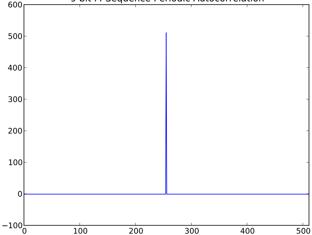
9 bit M-Sequence Periodic Autocorrelation
